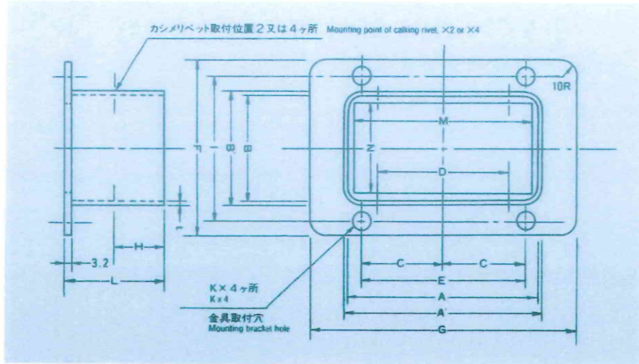
■取付け金具FF型寸法表 Mounting Bracket Size Table for FF Type
