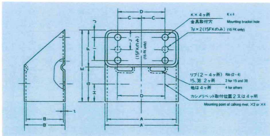
■取付け金具FK型寸法表 Mounting Bracket Size Table for FK Type
