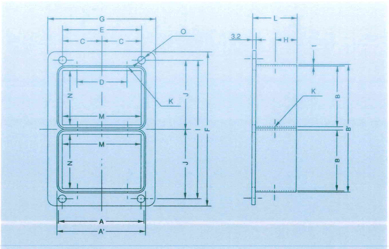
■取付け金具FFW型寸法表 Mounting Bracket Size Table for FFW
